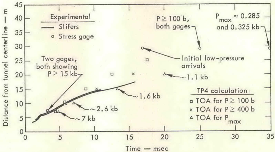
Fig. 16. Free-field measurements and calculated results for the vertical instrumentation hole.
