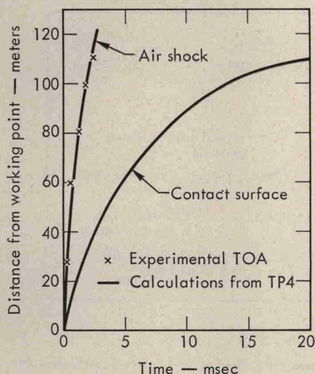
Fig. 17. Air-shock and contact-surface time of arrival.
